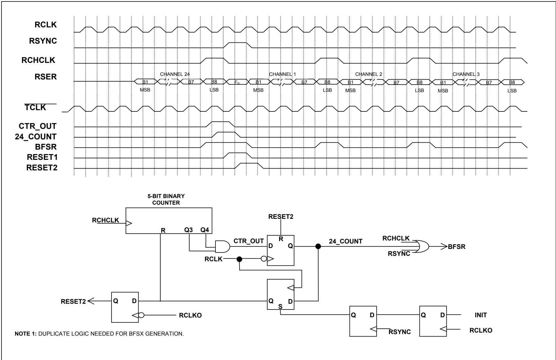
Figure 6. Generating BFSR 1 for Proper Burst Mode Operation of the TMS320C54x—T1 Clocking
