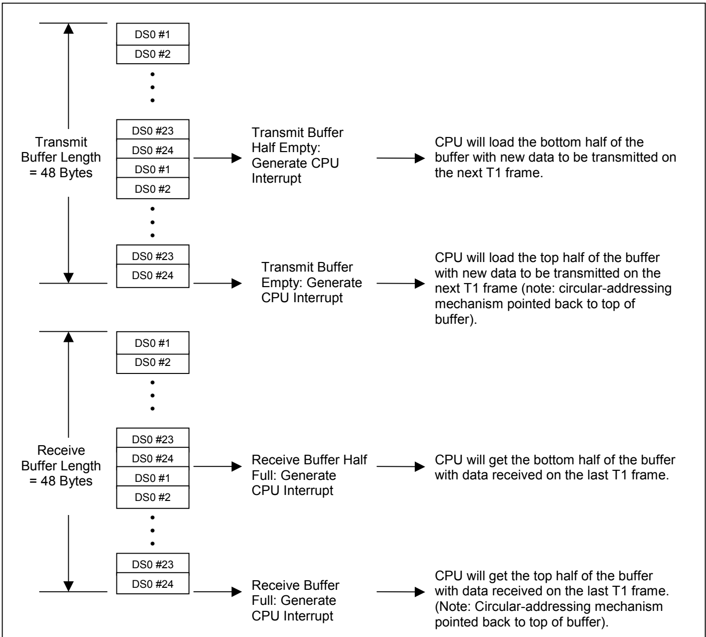
Figure 8. Autobuffering Unit Operation
