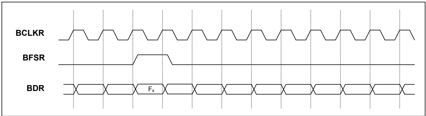
Figure 2. Continuous Mode Receive Timing (External Frame)
