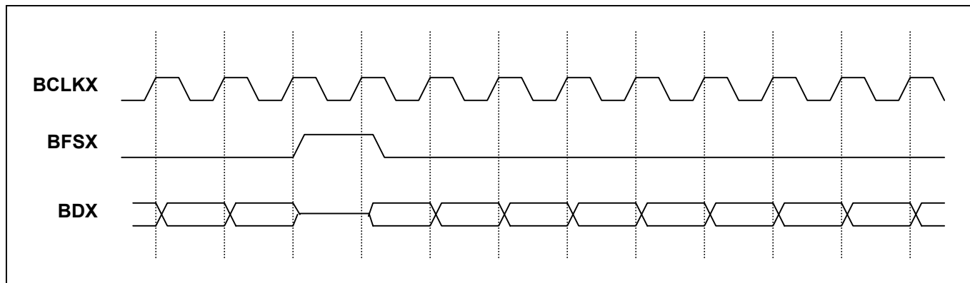
Figure 1. Continuous Mode Transmit Timing (External Frame)
