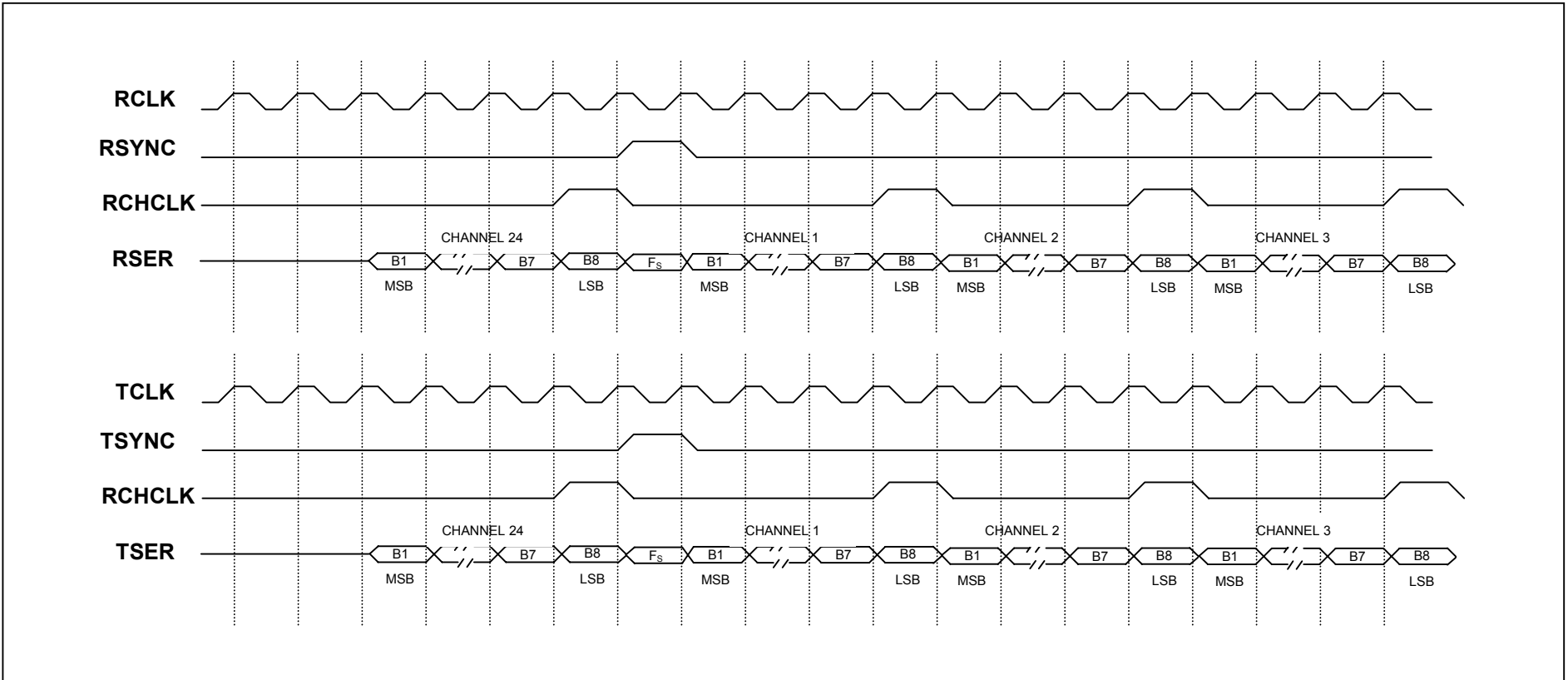
Figure 5. Timing Strobes Available on the DS21x52—T1 Timing
