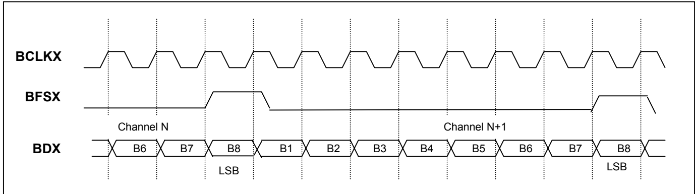
Figure 3. Burst Mode Transmit Timing (External Frame)
