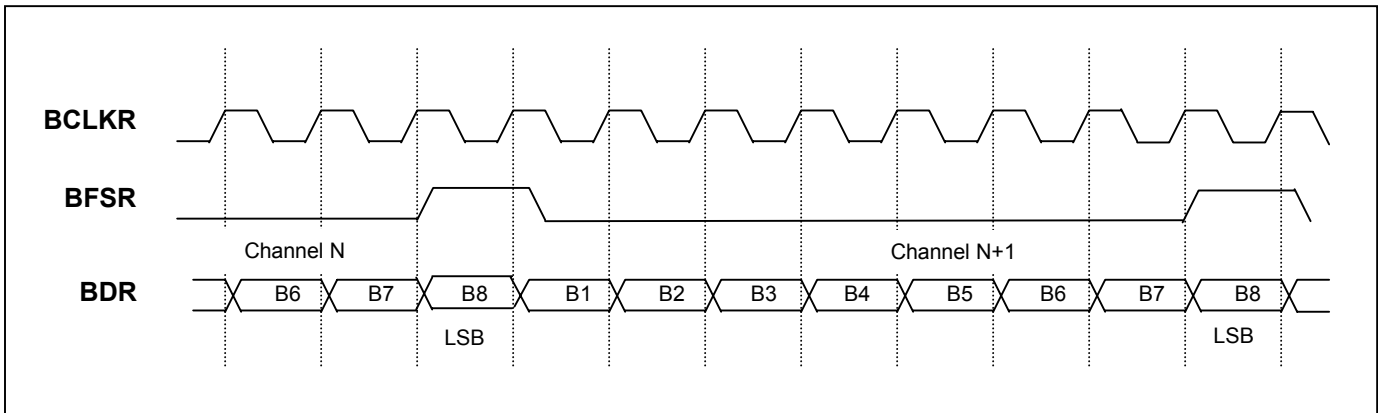
Figure 4. Burst Mode Receive Timing (External Frame)
